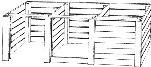
Figure 3. Redwood slat, three-bin composting unit.
