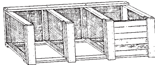
Figure 4. Redwood slat, hardware screen, three-bin composting unit.
