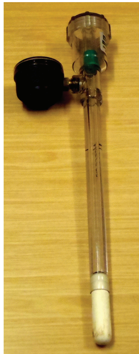
Figure 1. Tensiometer for measuring soil moisture tension.
